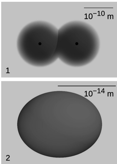
c / 1. The molecule N_2 . 2. The nucleus ^{178}\text{Hf} .
